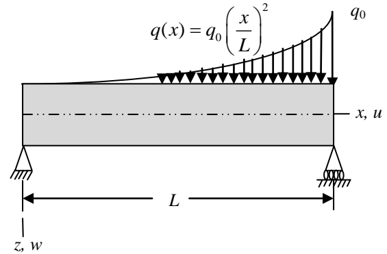
Fig. 2 Simply supported beam with parabolic load
