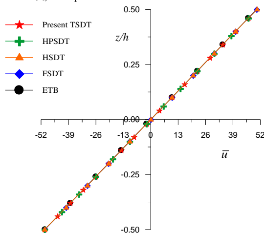
Fig. 4 Variation of axial displacement ( \bar{u} ) through the thickness beam at (x = 0.75L, z = 0) for aspect ratio 10.
