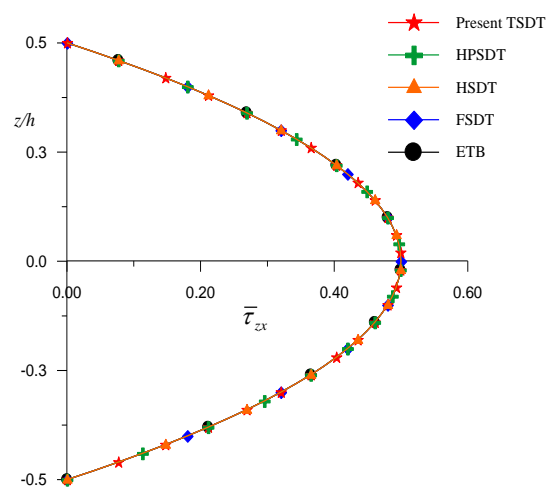
Fig. 10 Variation of transverse shear stress ( \bar{\tau}_{zx} ) through the thickness of beam at ( x = 0, z ) obtain using equilibrium equation for aspect ratio 4.
