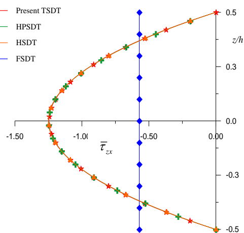
Fig. 9 Variation of transverse shear stress ( \bar{\tau}_{zx} ) through the thickness of beam at ( x = 0, z ) obtain using constitutive relation for aspect ratio 4.
