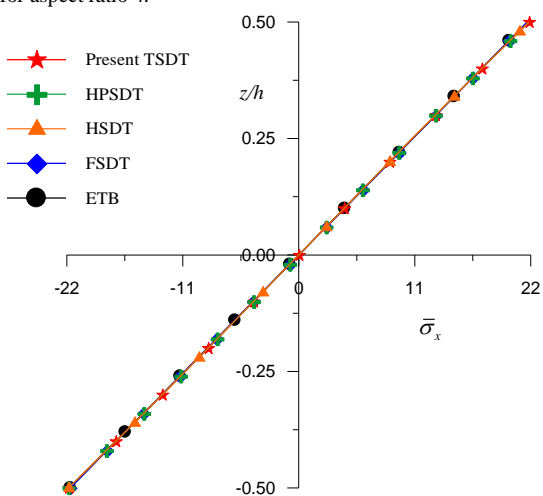
Fig. 6 Variation of axial stress ( \bar{\sigma}_x ) through the thickness beam at ( x = 0.75L, z ) for aspect ratio 4.
