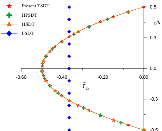
Fig. 8 Variation of transverse shear stress ( \bar{\tau}_{zx} ) through the thickness of beam at ( x = 0, z ) obtain using constitutive relation for aspect ratio 4.
