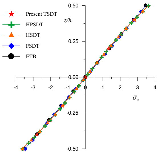
Fig. 6 Variation of axial stress ( \bar{\sigma}_x ) through the thickness beam at ( x = 0.75L, z ) for aspect ratio 4.
