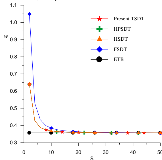
Fig. 5 Variation of maximum transverse displacement ( \bar{w} ) of beam at (x = 0.75L, z = 0) with aspect ratio S . (Example 1)
