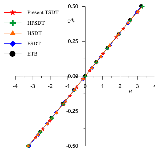
Fig. 3 Variation of axial displacement ( \bar{u} ) through the thickness of beam at (x = 0.75L, z) for aspect ratio 4.
