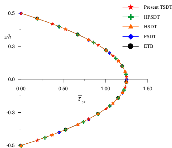
Fig. 10 Variation of transverse shear stress ( \bar{\tau}_{zx} ) through the thickness of beam at ( x = 0, z ) obtain using equilibrium equation for aspect ratio 4.
